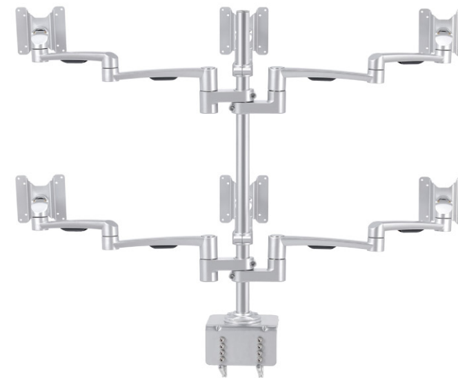
FA-518-1 VESA 75/100mm max ~36kg (79.2lbs)
